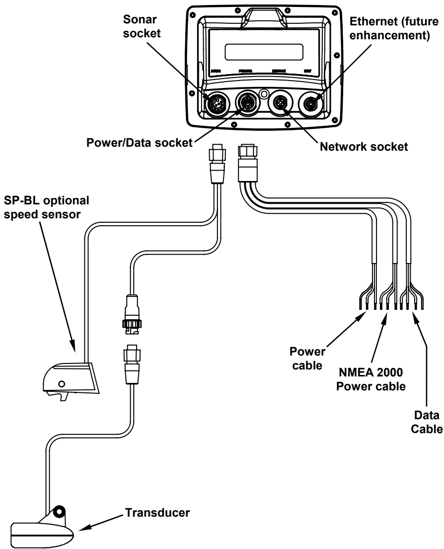
LMS-522c and LMS-527cDF cable connections.
