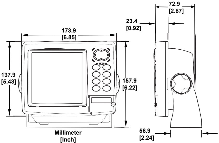
Front view (left) and side view (right) showing dimensions of the LMS-522c and LMS-527cDF sonar/GPS units mounted on gimbal bracket.
